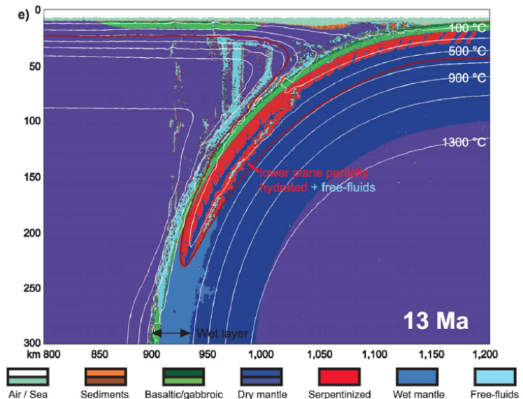
Figure 1 – Numerical modelling of slab hydration at the trench outer-rise due to bending-related faulting and subsequent dehydration at upper mantle depths. From (Faccenda et al. 2012)
