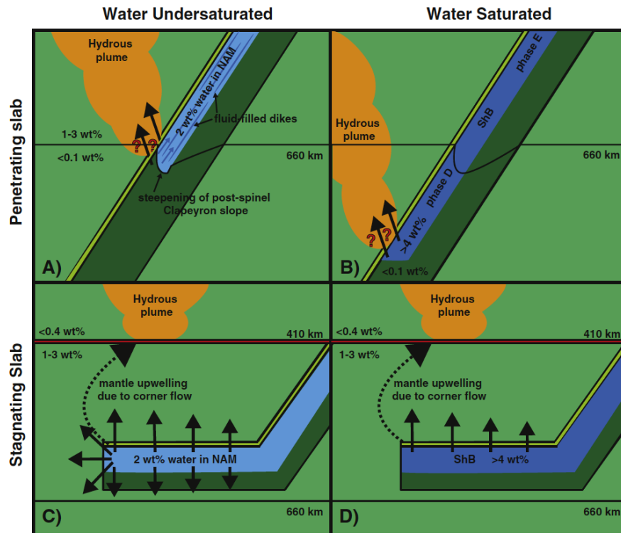
Figure 2 – Hypothetical models of deep slab mantle dehydration in H_2O -undersaturated and H_2O -saturated conditions for penetrating and stagnating slabs. Dark blue is hydrated mantle, light blue is wet mantle. Red indicates partially molten mantle, while orange is representative of upwelling hydrous plumes. Light and dark green are the ambient and lithospheric mantle. NAM are nominally anhydrous minerals. Phase E, ShB, D are deep hydrous phases. Values in wt% indicate mantle water contents. From (Faccenda, 2014).
